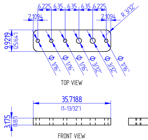
UPPER POST PLATE Quantity: 2
