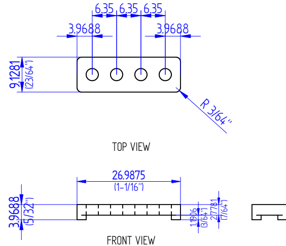
LOWER POST PLATE Quantity: 2
